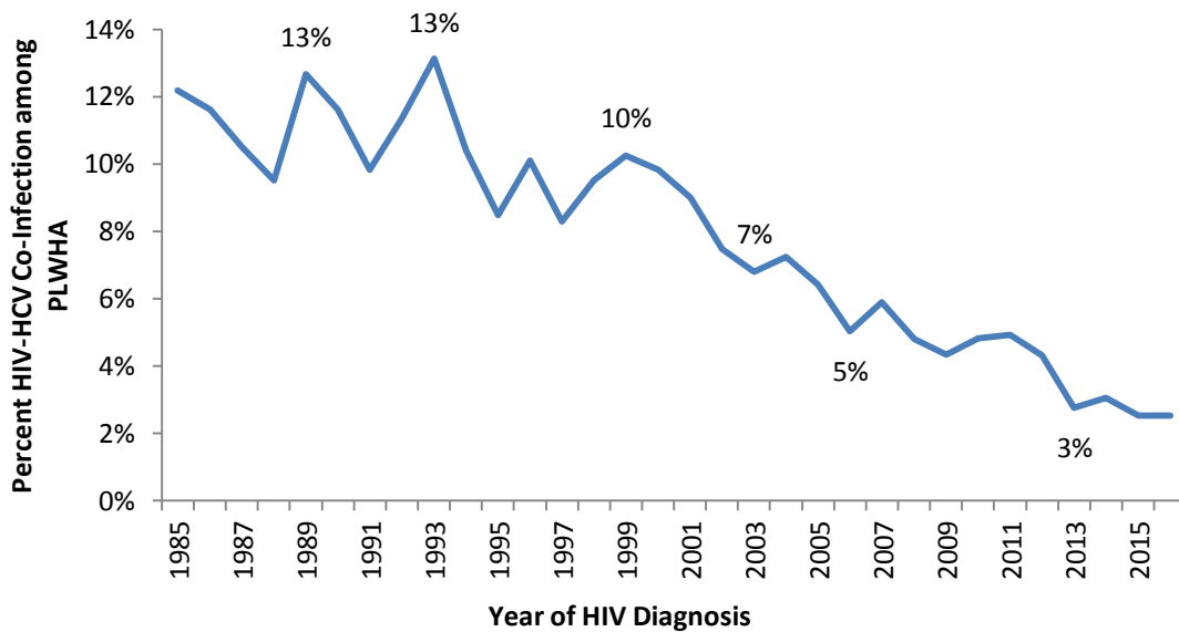
Figure 3. Percent PLWHA Co-Infected with HCV by Year of HIV Diagnosis, Illinois, 1985–June, 2016
