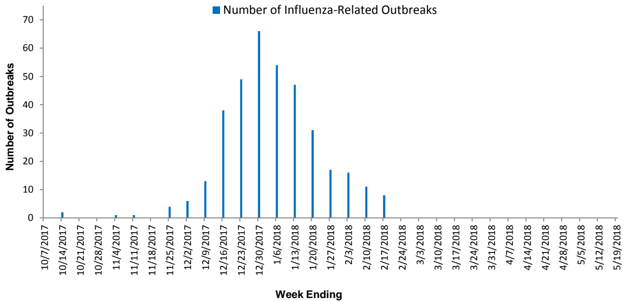
Influenza Outbreaks by First Onset Date, Illinois, 2017-2018
